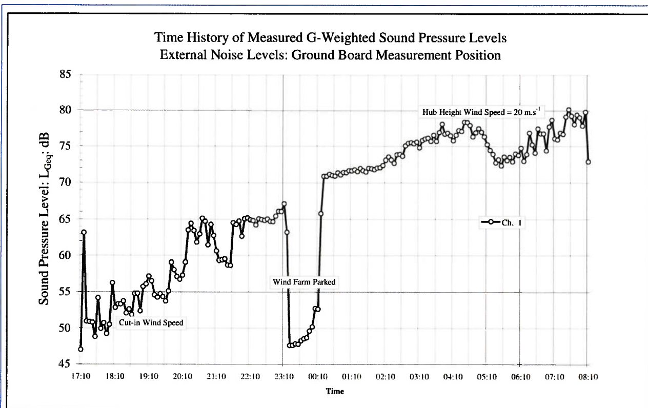
Figure 12: Time History Figure of G-Weighted Sound Pressure Levels for a Wind Farm
